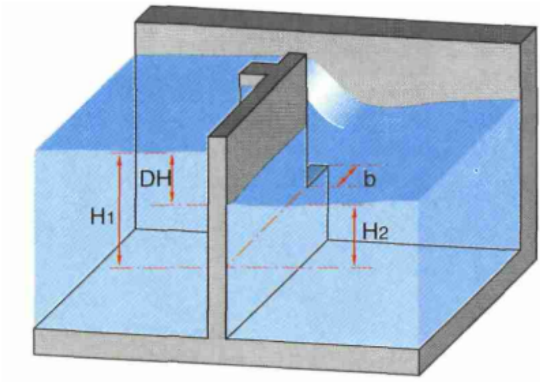
Figure 1.15: Notch diagram
