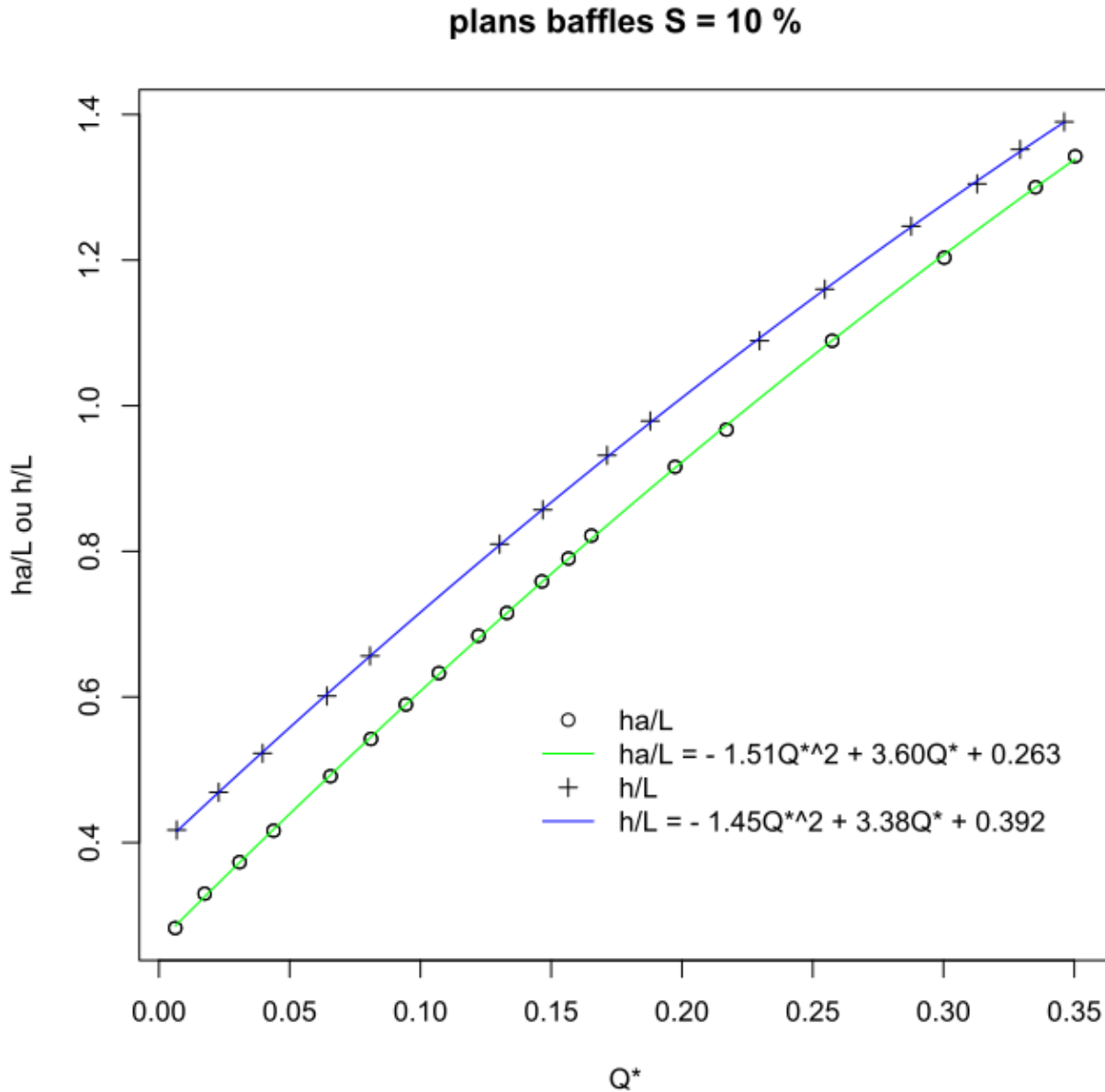
Figure 1.42: Abacuses of a plane baffles (Denil) fishway for a slope of 10%
