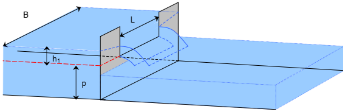
Figure 1.16: Kindsvater-Carter formula: weir diagram
