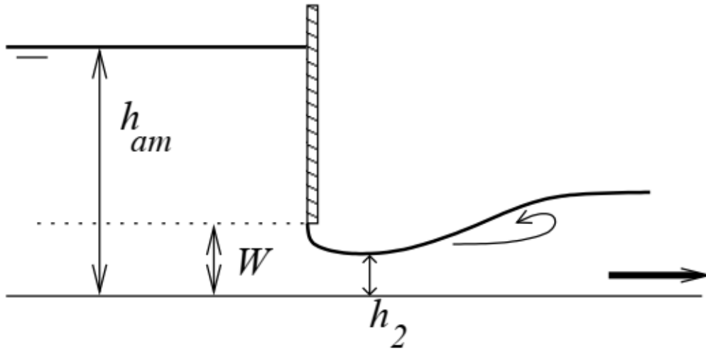
Figure 1.31: Free flow sluice gate diagram
