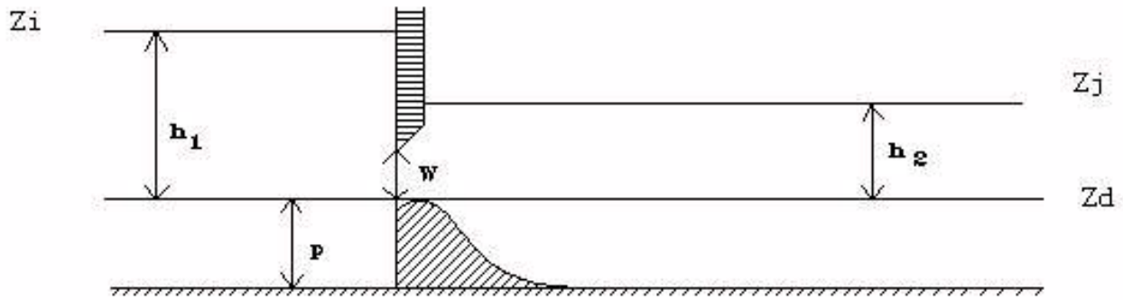
Figure 1.27: CEM 88 V diagram
