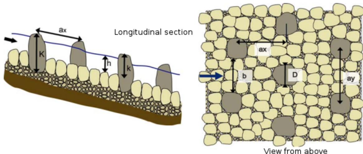
Figure 1.38: Schematic of a regular arrangement of rockfill and notations
