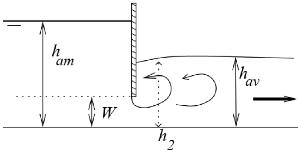
Figure 1.32: Submerged gate diagram
