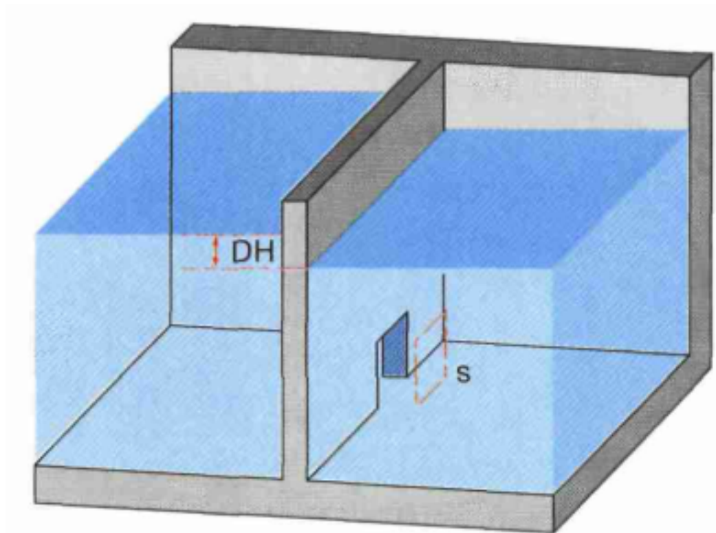
Figure 1.34: Submerged orifice diagram
