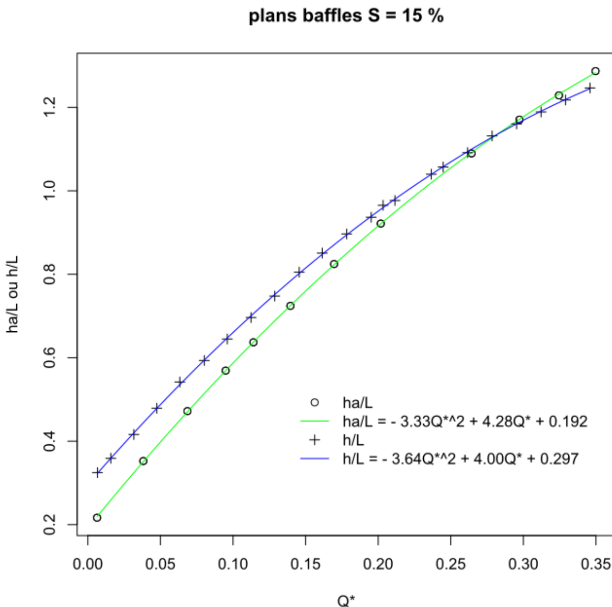
Figure 1.43: Abacuses of a plane baffles (Denil) fishway for a slope of 15%
