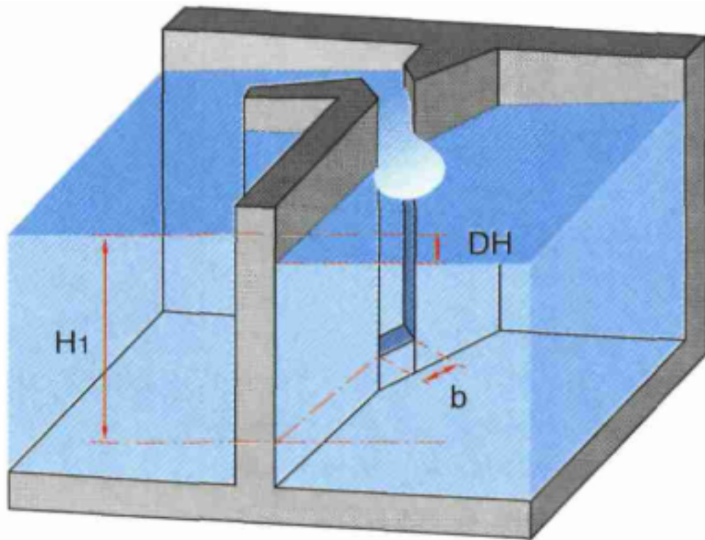
Figure 1.21: Submerged slot diagram
