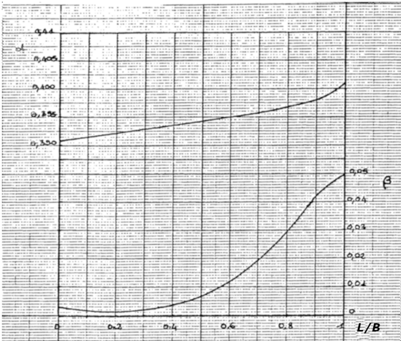
Figure 1.17: Kindsvater-Carter formula: abacuses
