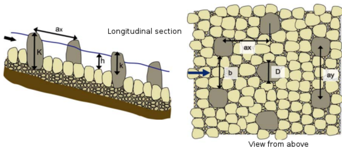
Figure 1.40: Schematic of a regular arrangement of rockfill and notations
