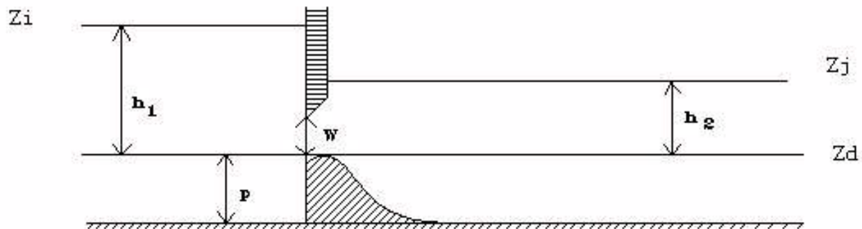
Figure 1.29: CEM 88 D diagram
