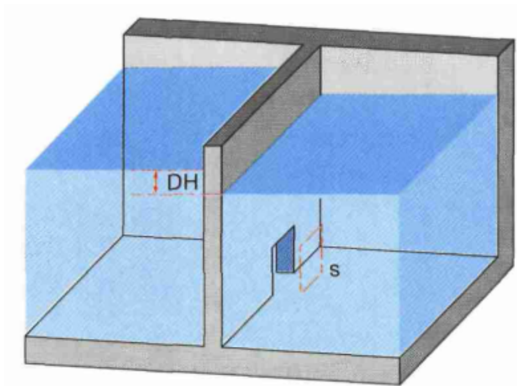
Figure 1.13: Submerged orifice diagram
