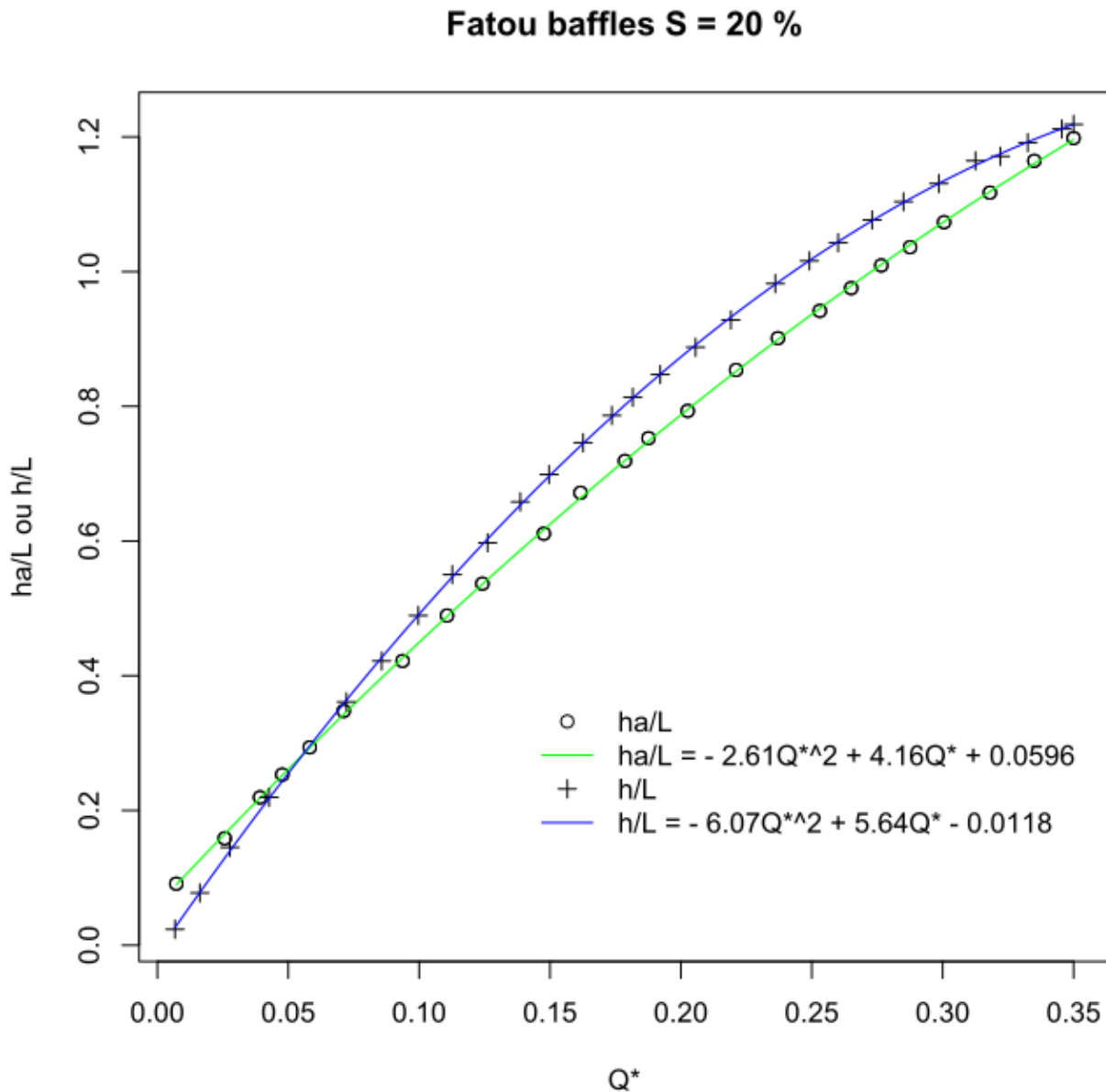
Figure 1.48: Abacuses of a Fatou baffle fishway for a slope of 20%
