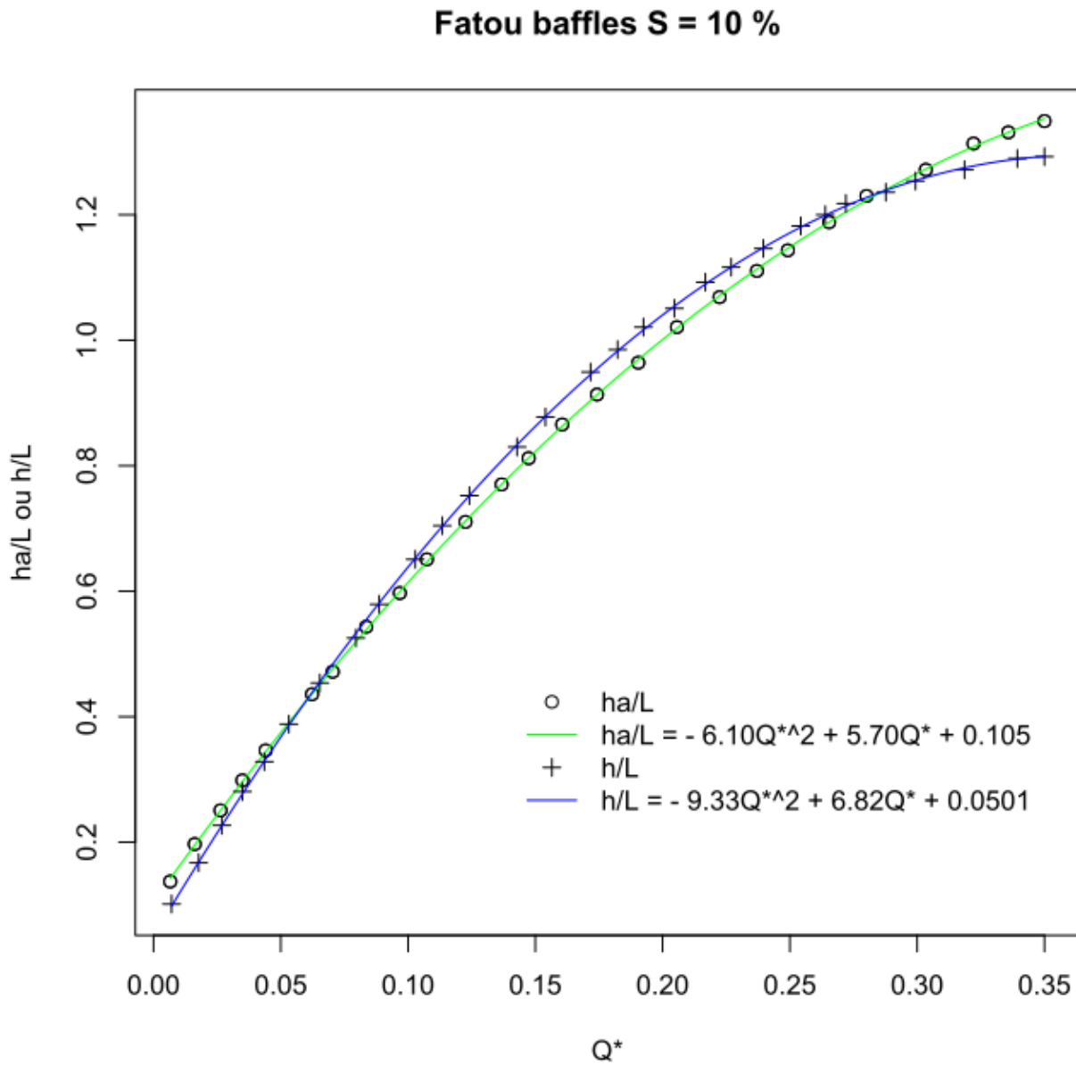
Figure 1.46: Abacuses of a Fatou baffle fishway for a slope of 10%
