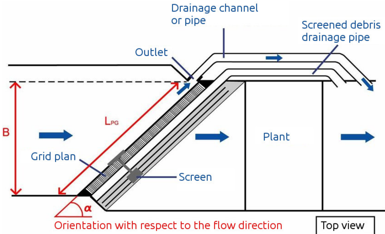
Figure 1.55: Angled trashrack
