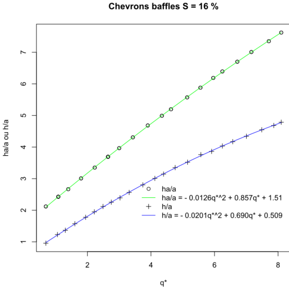
Figure 1.54: Abacuses of a mixed / chevron baffles fishway for a slope of 16%
