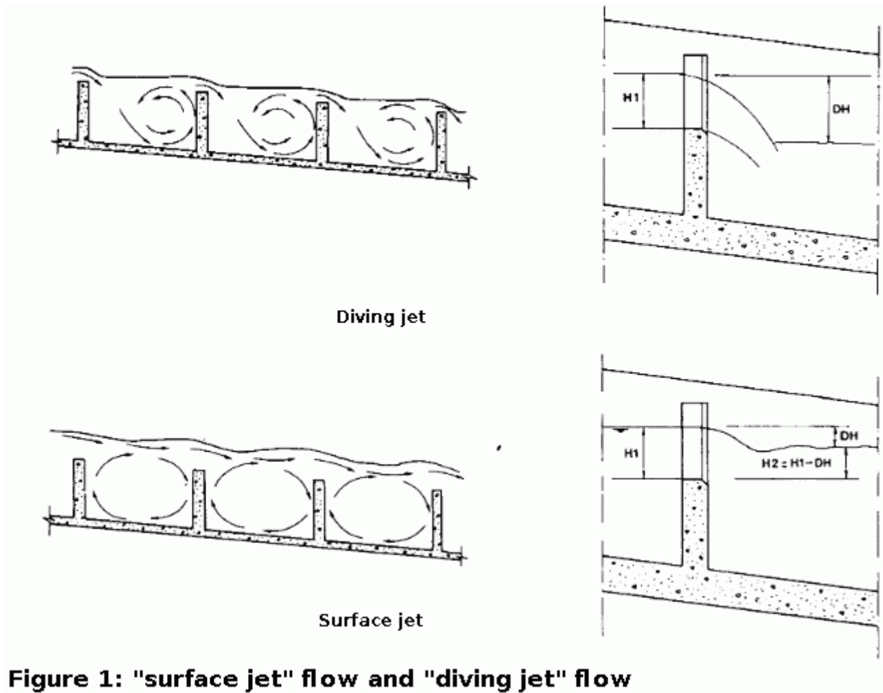
Figure 1.12: Diagram of jet type
