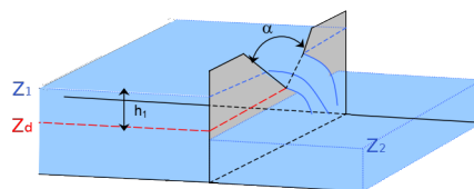
Figure 1.25: Perspective view of a triangular weir
