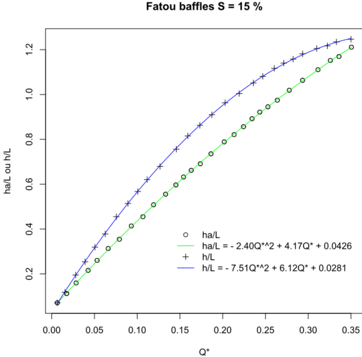
Figure 1.47: Abacuses of a Fatou baffle fishway for a slope of 15%
