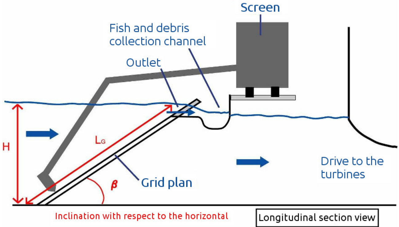
Figure 1.57: Inclined trashrack
