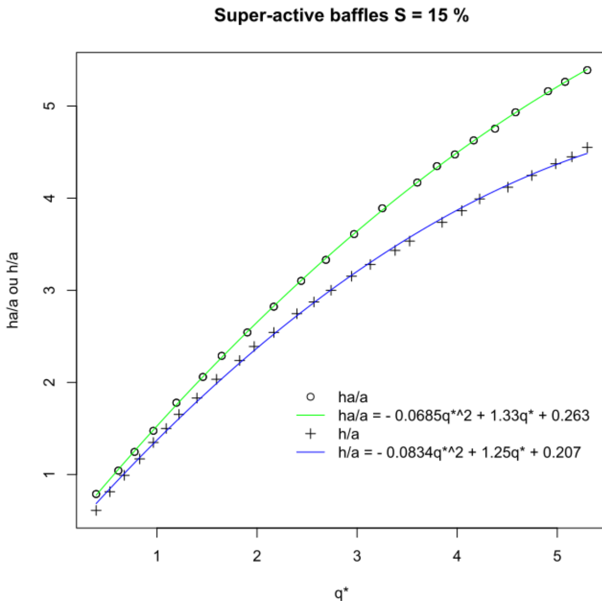
Figure 1.51: Abacuses of a superactive baffles fishway for a slope of 15%
