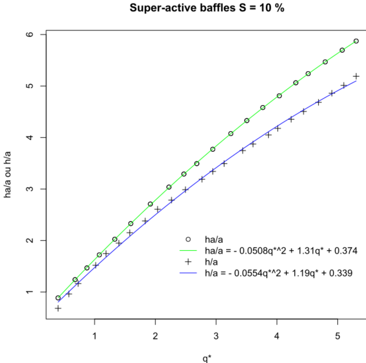
Figure 1.50: Abacuses of a superactive baffles fishway for a slope of 10%
