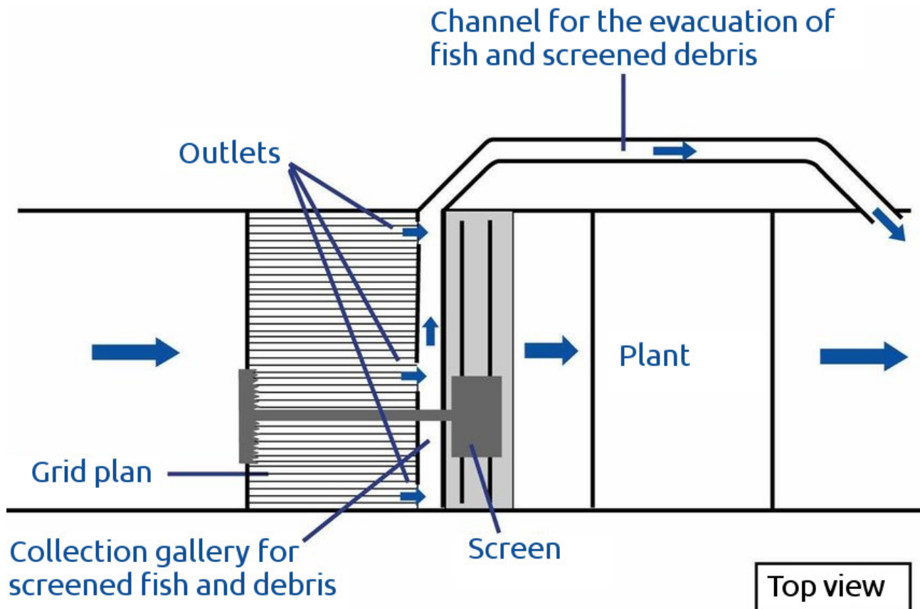
Figure 1.56: Inclined trashrack
