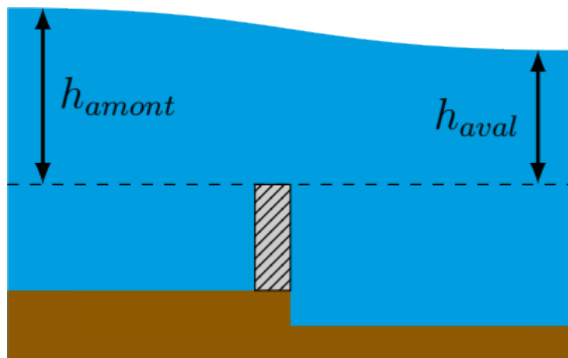
Figure 1.24: Submerged weir diagram
