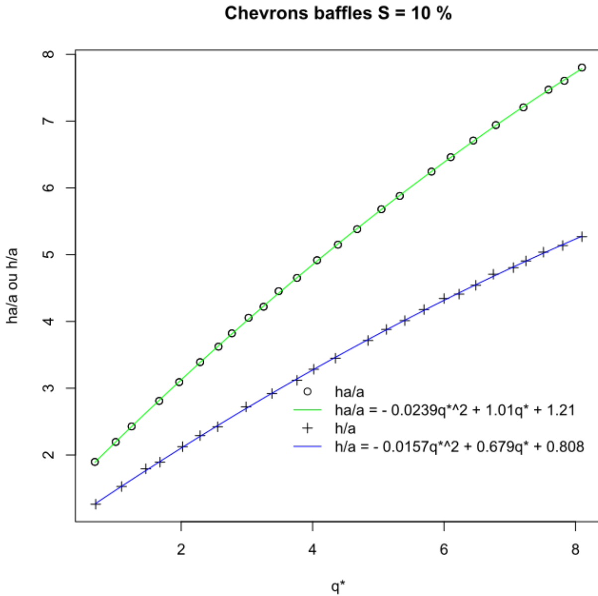
Figure 1.53: Abacuses of a mixed / chevron baffles fishway for a slope of 10%
