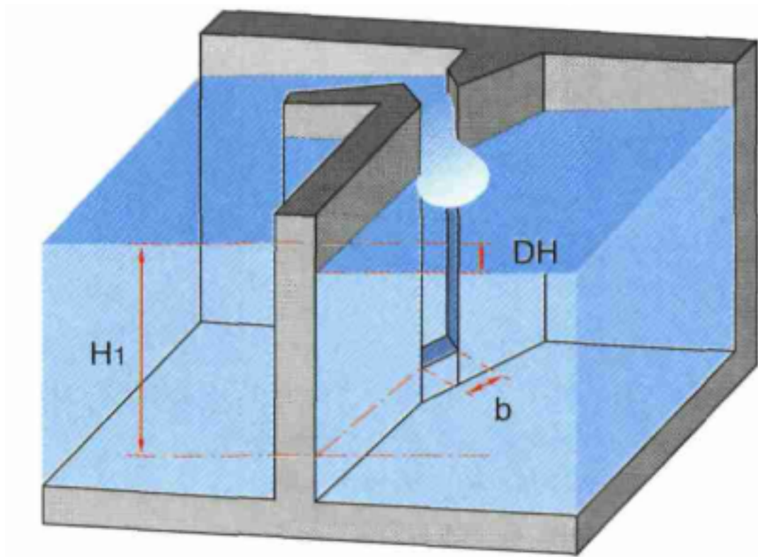
Figure 1.35: Schematic of the submerged slot
