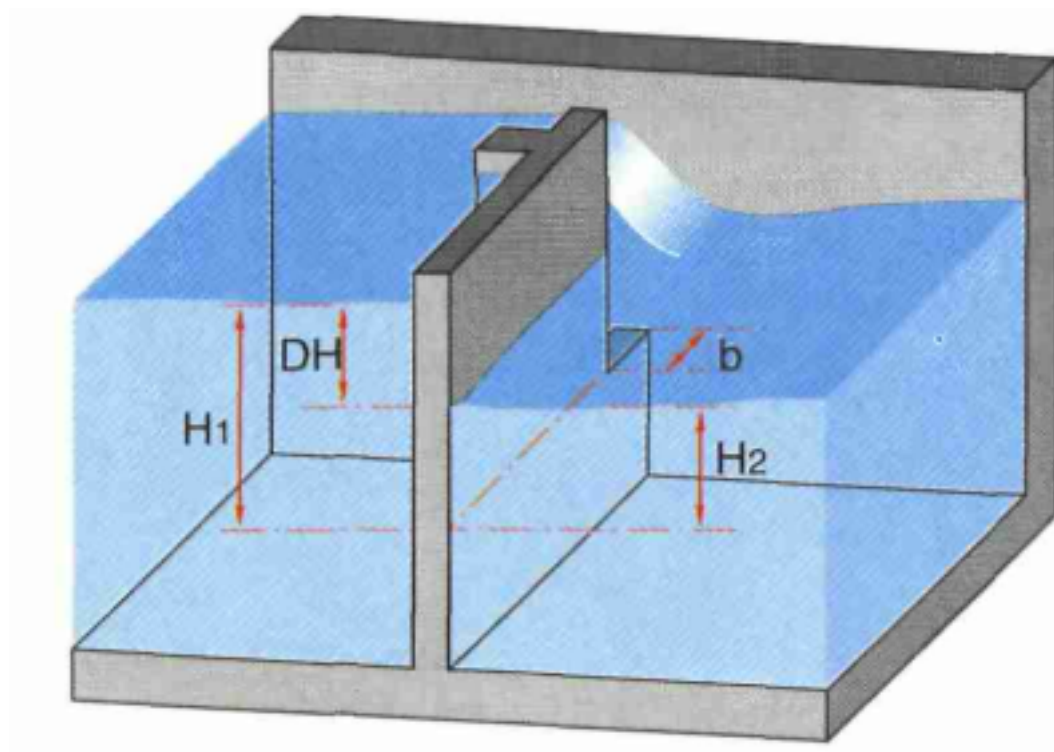
Figure 1.36: Notch diagram
