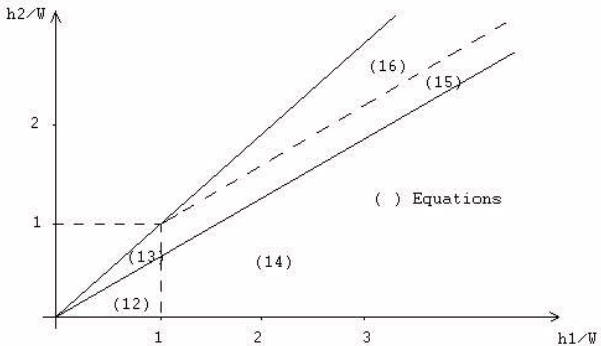
Figure 1.30: CEM 88 D chart
