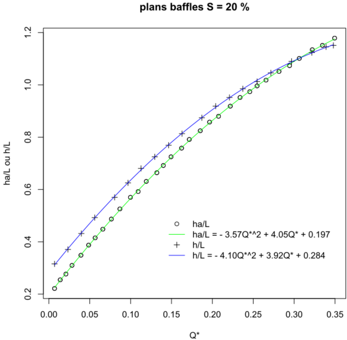
Figure 1.44: Abacuses of a plane baffles (Denil) fishway for a slope of 20%
