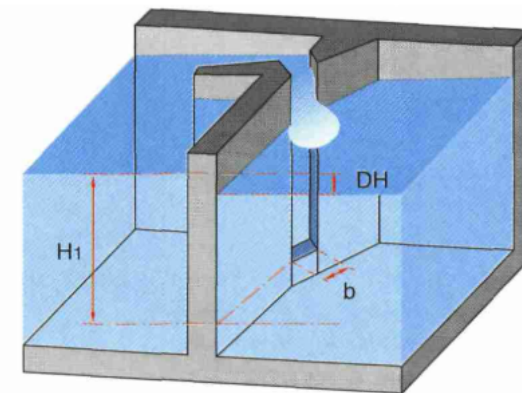
Figure 1.14: Schematic of the submerged slot
