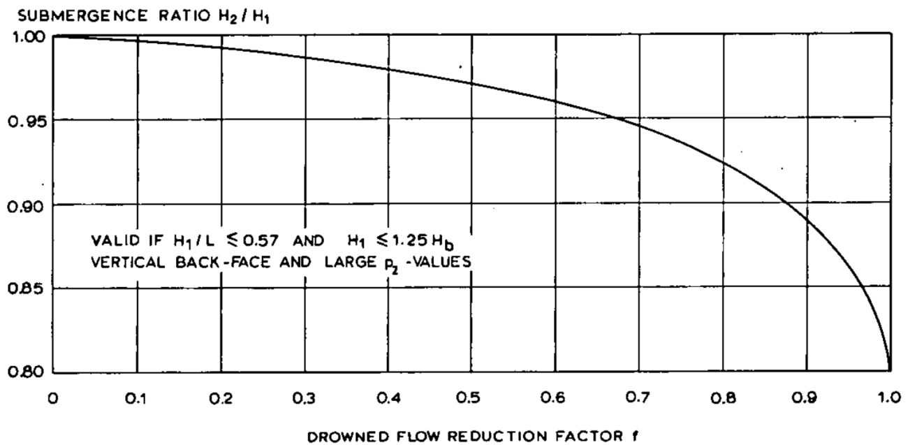
Figure 1.26: Submergence reduction factor for a V-notch broad-crested weir (from Bos, 1989 5) )
